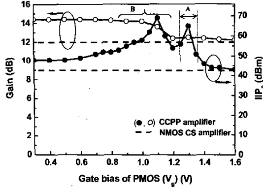
Fig. 3. Measured gain and IIP 2 of CCPP amplifier and NMOS common source (CS) amplifier (Solid and dashed lines are for CCPP and NMOS CS amplifier, respectively. Power supply voltage is 1.8V.)
